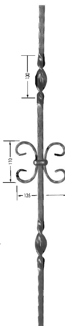
4-5013 L: 950 mm. Ø 14 mm.
