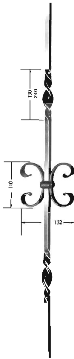
4-2013 L: 950 mm. ∅ 12 mm.
