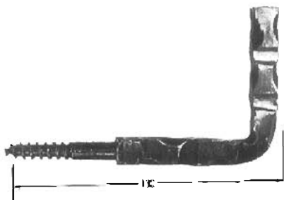
4-8410 M \square :14 x 14 mm. L: 130 mm.
